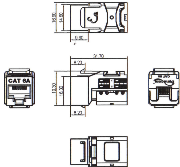
ASSEMBLY DIMENSION
