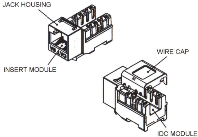
ISOMETRIC VIEW
